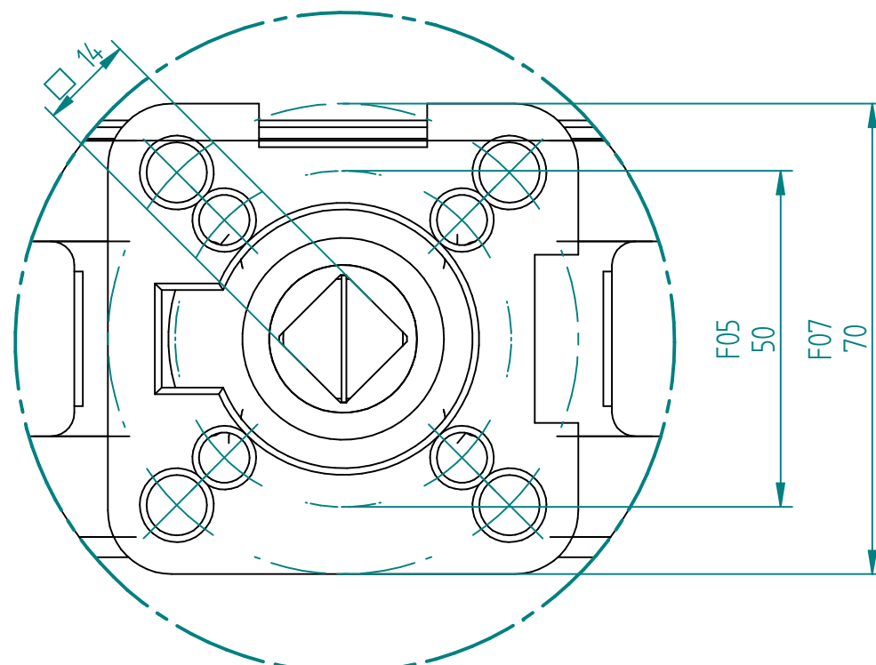
DETAIL A
