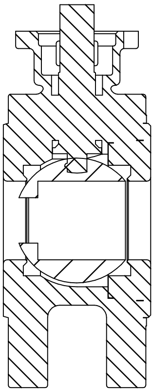
SECTION B-B
