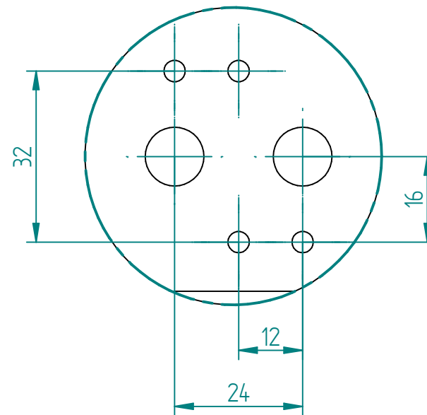
DETAIL A 1:1 Hole pattern for solenoid valves acc. to VDI/VDE 3845, NAMUR
