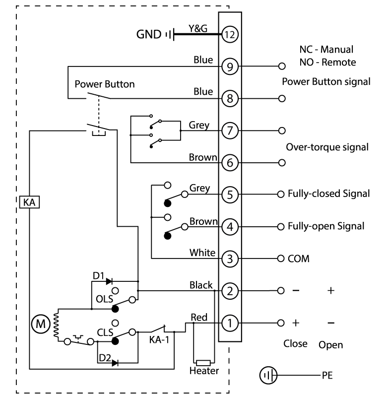
GD-TYPE WIRING CIRCUIT
