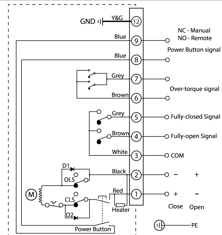
GD-TYPE WIRING CIRCUIT
