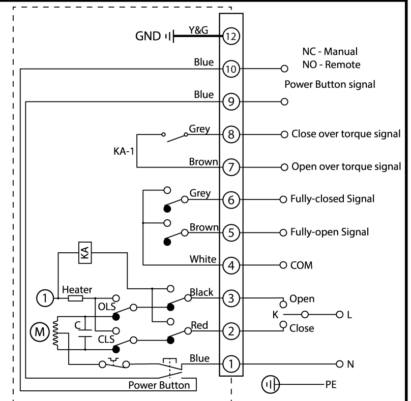
BD-TYPE WIRING CIRCUIT
