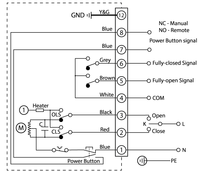
BD-TYPE WIRING CIRCUIT
