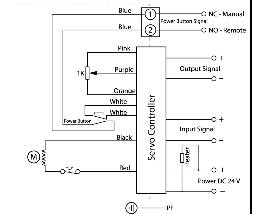
GEYD-TYPE WIRING CIRCUIT
