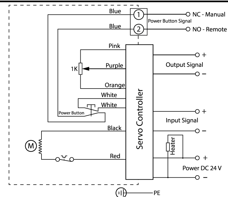
GEYD-TYPE WIRING CIRCUIT
