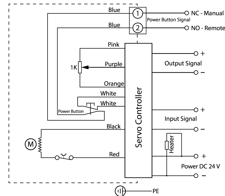
GEYD-TYPE WIRING CIRCUIT
