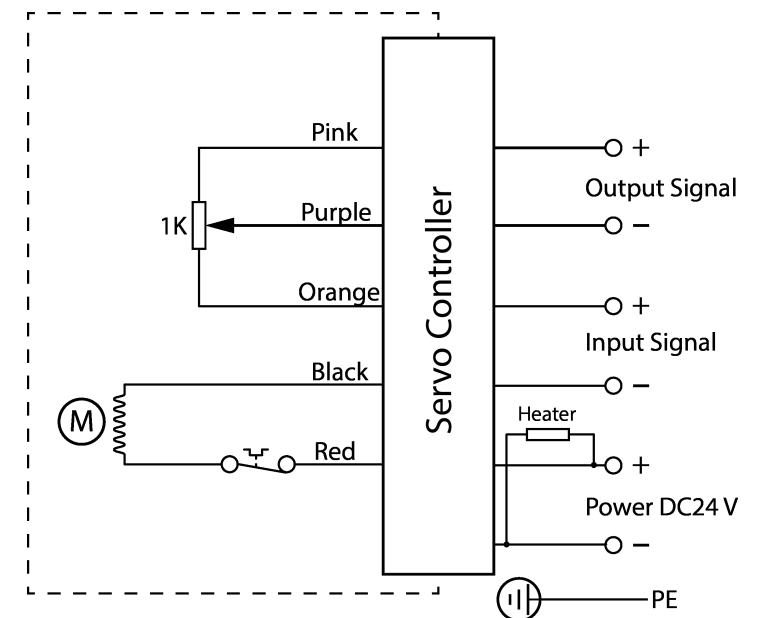
GEY-TYPE WIRING CIRCUIT
