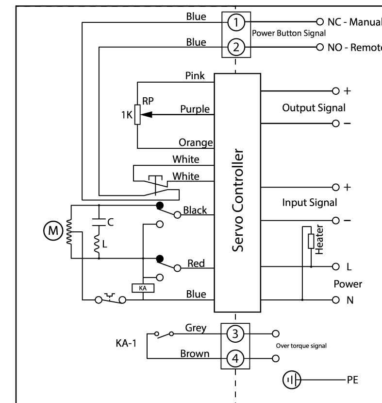
ED-TYPE WIRING CIRCUIT
