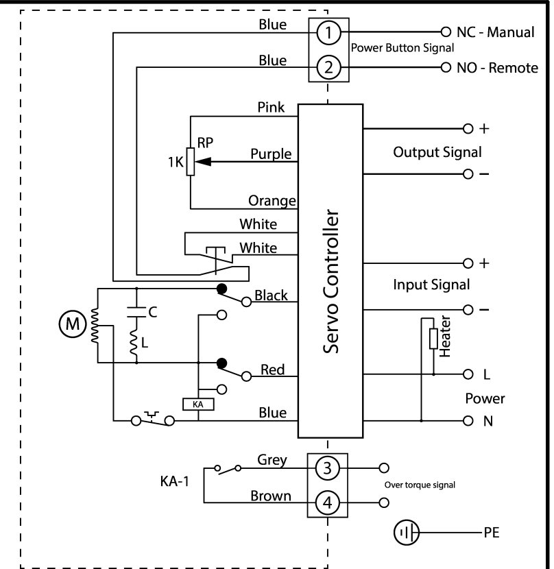
ED-TYPE WIRING CIRCUIT
