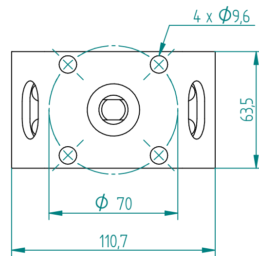
1:2 Mounting Plate
