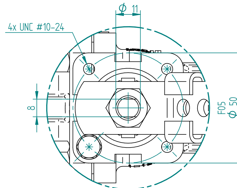
DETAIL A
