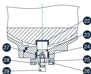
B VIEW
