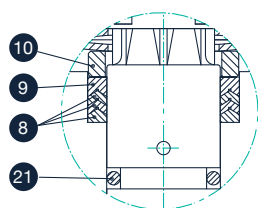
A VIEW
