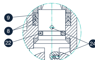
A VIEW
