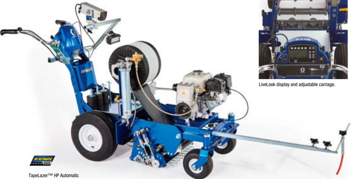
TapeLazer™ HP Automatic (unit shown includes optional LazerGuide 3000 and high-output LED light)
